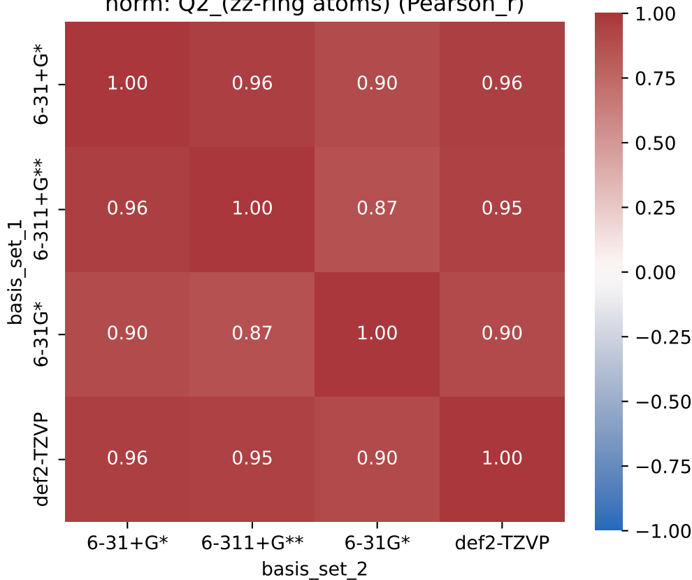
norm: Q2_(zz-ring atoms) (Pearson_r)
